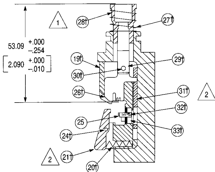
MTA-.100 Head Assembly 318862-1
