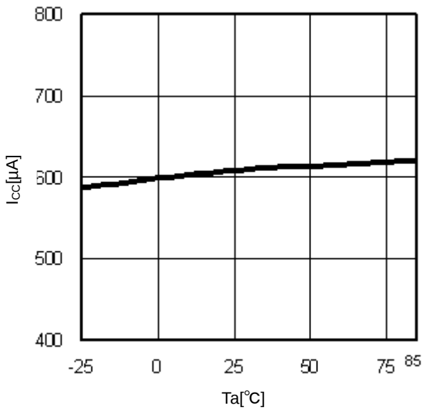
Figure 10. T_a - I_{cc}
