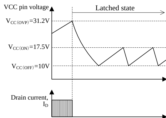
Figure 9-10 OVP operational waveforms
