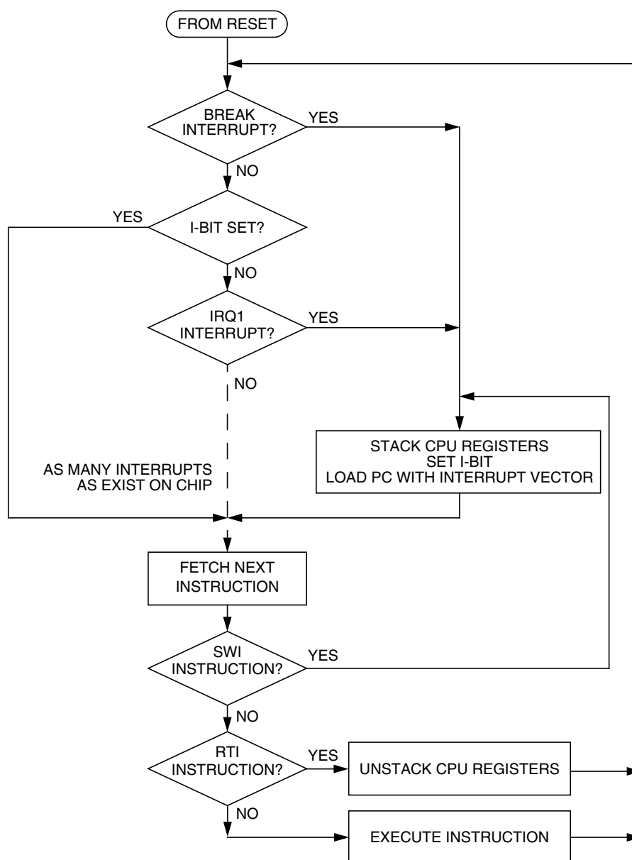
Figure 7-10. Interrupt Processing
