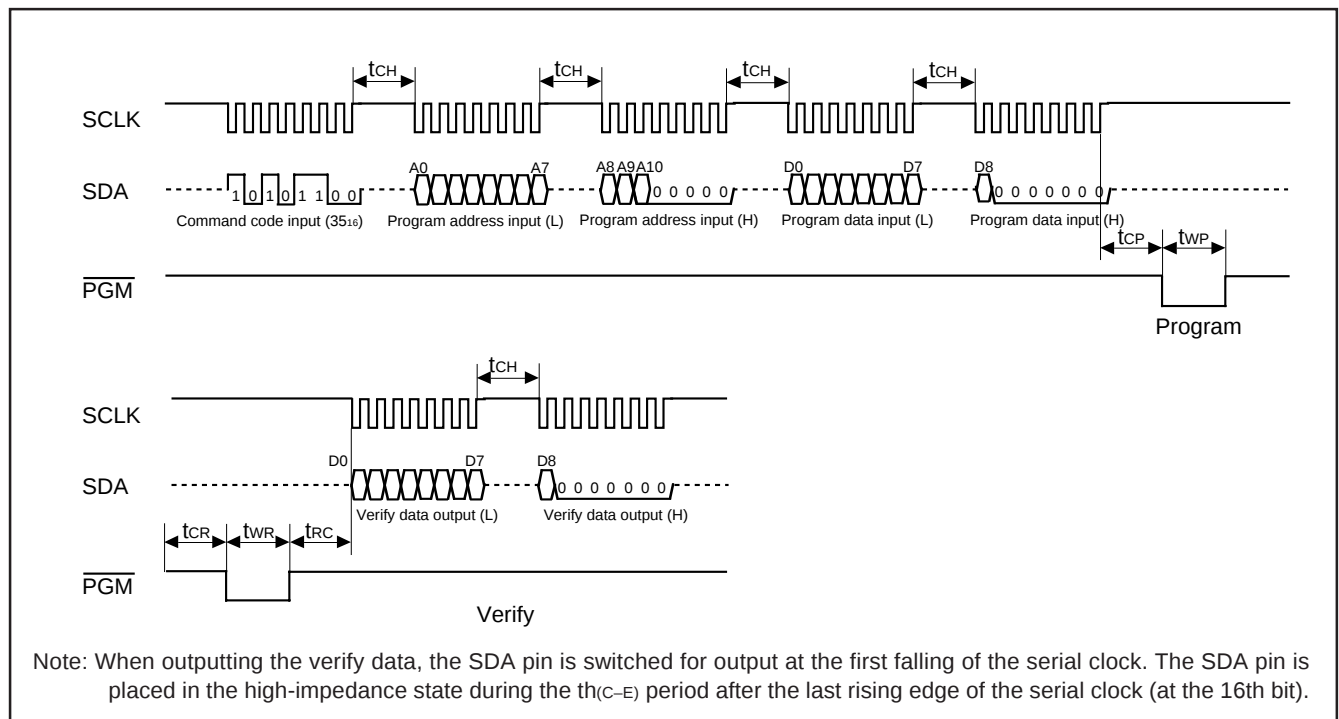
Fig. 33 Timing at program verifying
