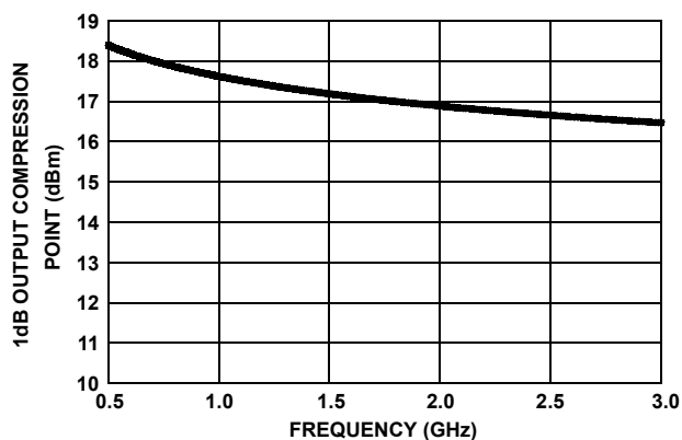
FIGURE 12. P1dB vs FREQUENCY
