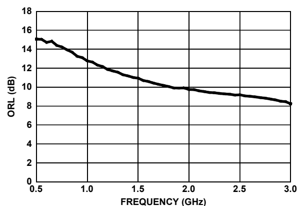
FIGURE 4. OUTPUT RETURN LOSS vs FREQUENCY
