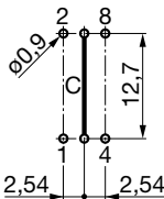
Drilling diagram View from component side
