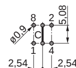
Drilling diagram View from component side
