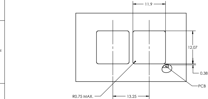
RECOMMENDED PANEL CUTOUT FOR SINGLE LEVEL MOUNTING
