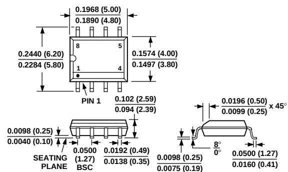
8-Lead Narrow SOIC (R-8)
