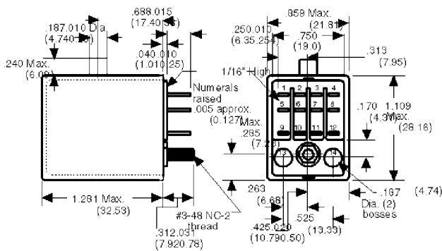
Dust Cover 158-1, 2
