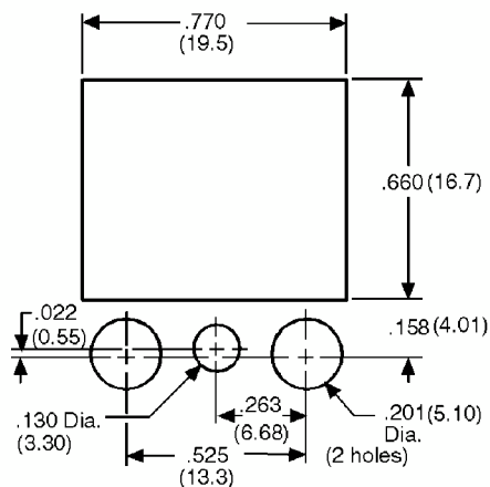
Model 158-1, -4
