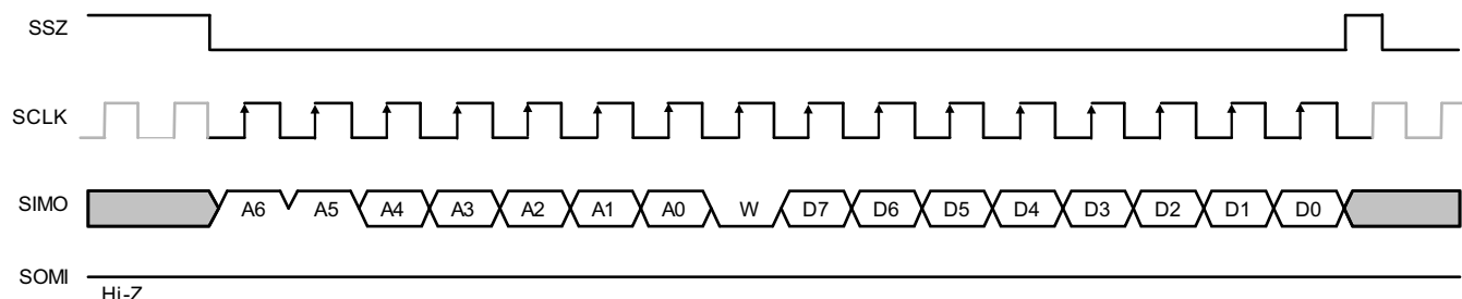
Figure 18. Write 8-Bits Control Register
