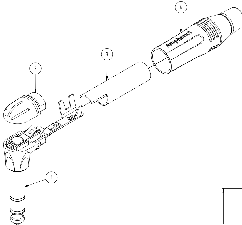
Stereo Connector Assembly - Parts List
