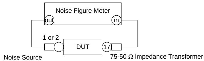
Figure 2: Noise Figure measurement
