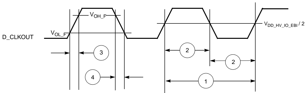
Figure 50. D_CLKOUT Timing
