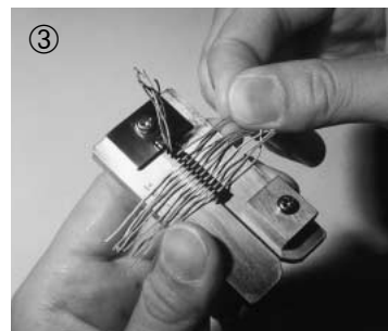
3. Arrange the wires one at a time through holding plates (A) and (B).
