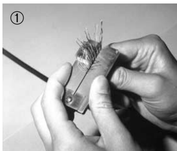
1. Set the wires in the wiring fixtures.
