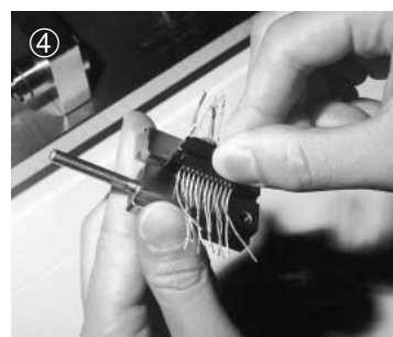
6. Pull down the handle. The wiring and cutting of excess cable length are completed.
