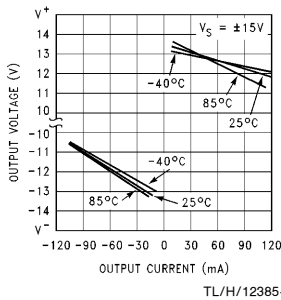
Output Voltage vs Output Current
