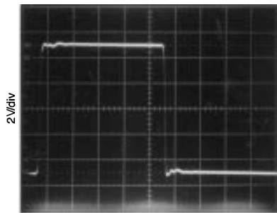
FIGURE 3. Properly Terminated Signal
