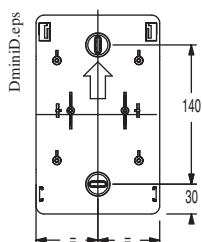
3, 4 and 6 modules
