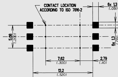
CCM04-5004*/1201/1202/1203/1204 PCB Layout
