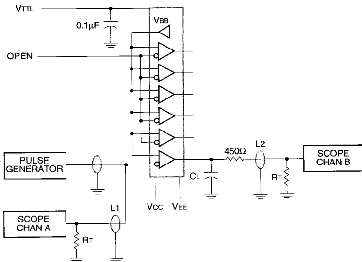
Figure 2. AC Test Circuit for 15pF Loading
