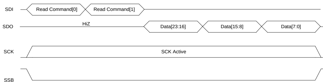
Figure 4-3: Single Word Read Access Timing
