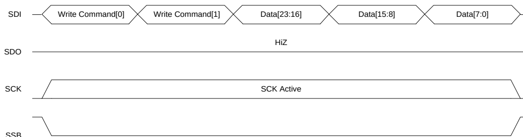
Figure 4-4: Single Word Write Access Timing
