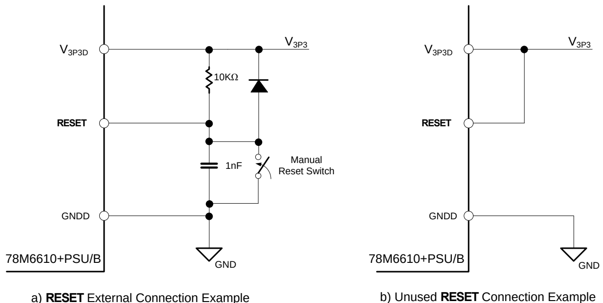
Figure 1-3: RESET Pin Connections
