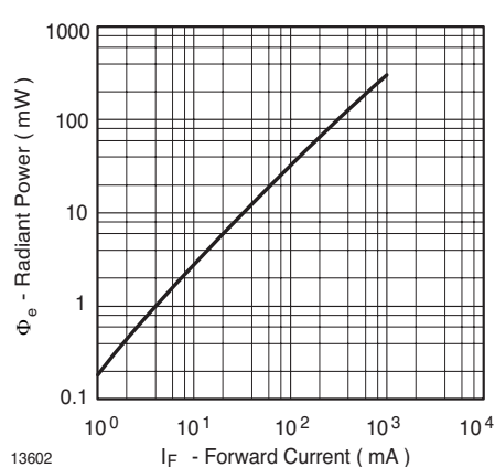
Figure 7. Radiant Power vs. Forward Current
