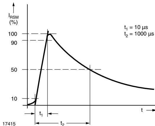
Fig. 4 - Pulse Waveform
