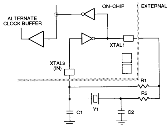
Figure 9. Direct Interconnect
