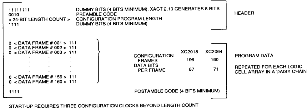
Figure 13. XC2064 Internal Configuration Data Arrangement
