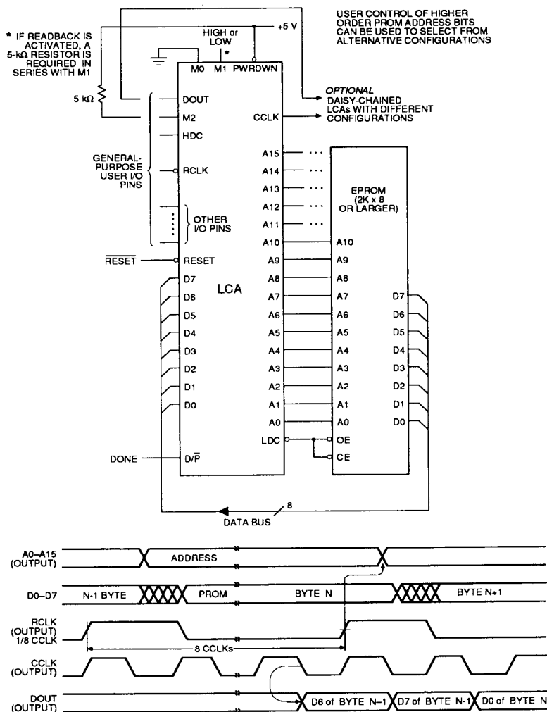
Figure 15a. Master Parallel Mode. Configuration data are loaded automatically from an external byte wide PROM. An XC2000 \overline{LDC} signal can provide a PROM inhibit as the user I/Os become active.
