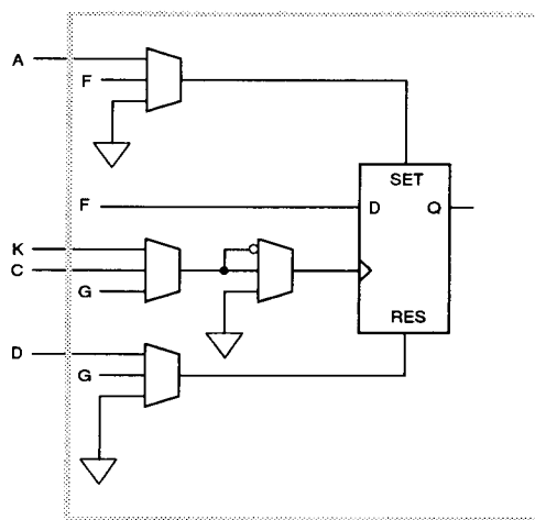
Figure 6. CLB Storage Element
