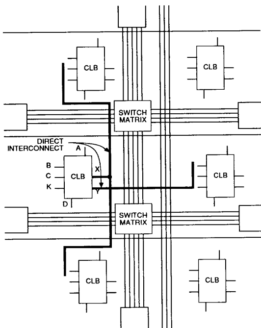
Figure 9. Direct Interconnect
