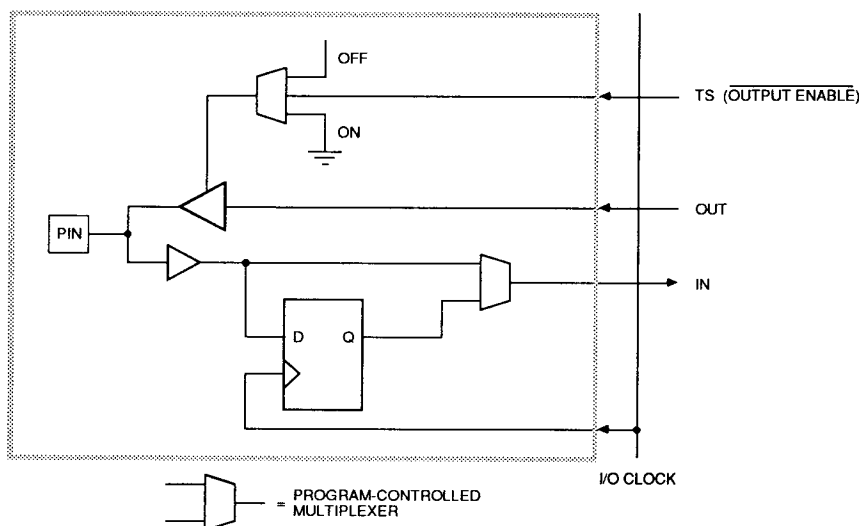
Figure 3. I/O Block
