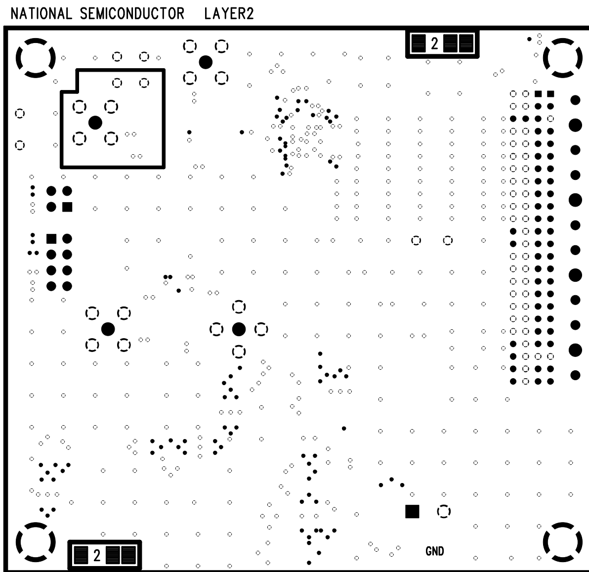
Figure 7. Layer 2 - Ground
