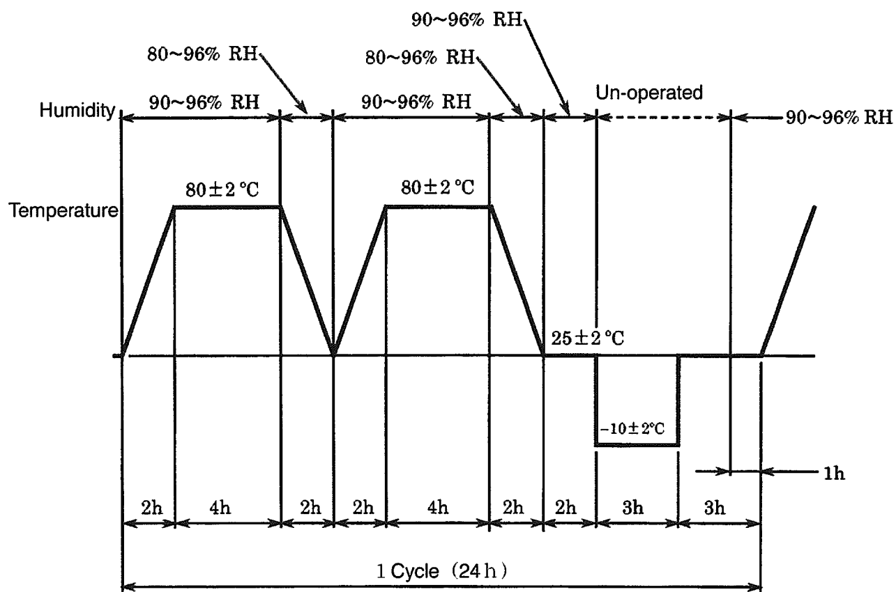
Fig. 9 Humidity-Temperature Cycling
