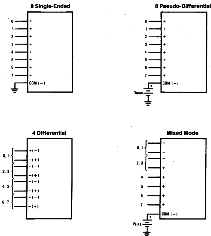
FIGURE 1. Analog Input Multiplexer Options for the ADC08038
