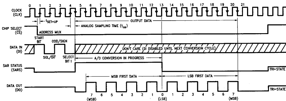
ADC08034 Timing
