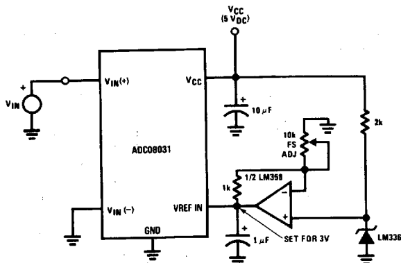
Span Adjust; 0V \leq V_{IN} \leq 3V
