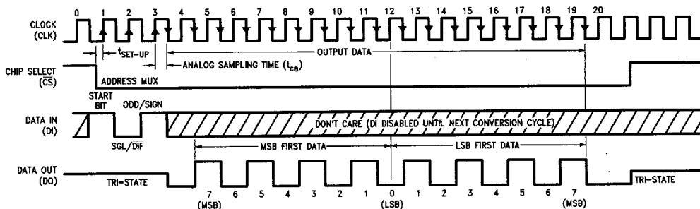
ADC08032 Timing
