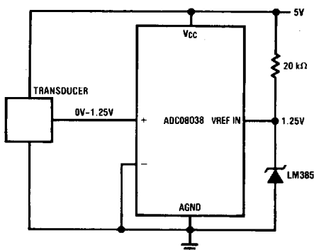
b) Absolute with a Reduced Span
