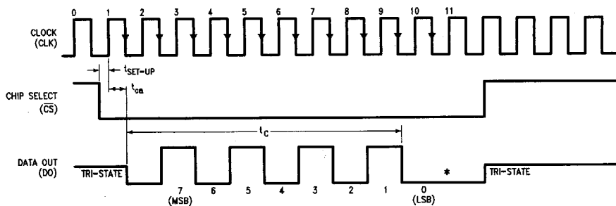
ADC08031 Timing
