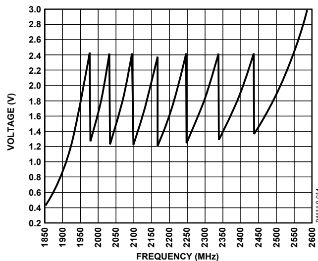
Figure 14. Frequency vs. V_{TUNE} ADF4360-1
