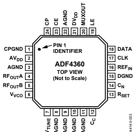
Figure 3. Pin Configuration
