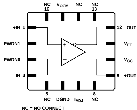
Figure 1. 4 mm \times 4 mm 16-Lead LFCSP
