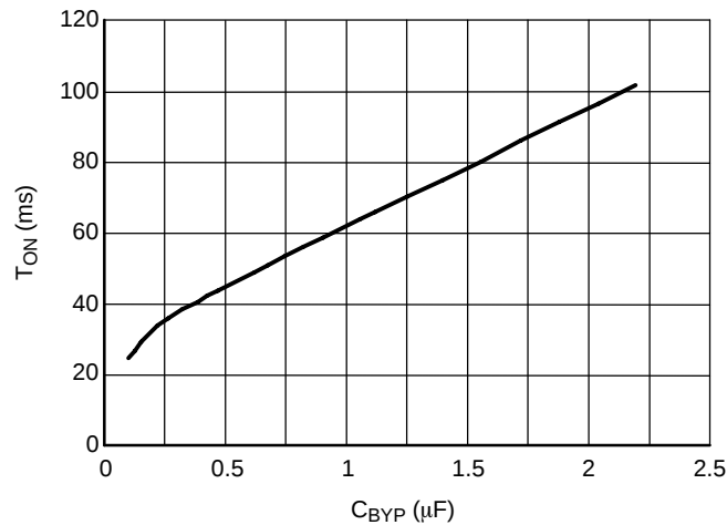
Figure 18. Turn On Time versus C_{BYF} @ V_{BAT} = 3.6 V, T_A = +25^\circ C , C_{IN} = 100 nF, R_{IN} = 22 k, R_F = 110 k
