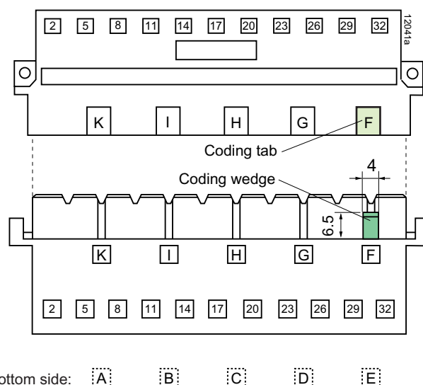
Fig. 17 Integrated code key system (H15 connector)
