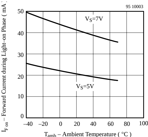
Figure 4. Forward Current (Light On) vs. Amb. Temperature
