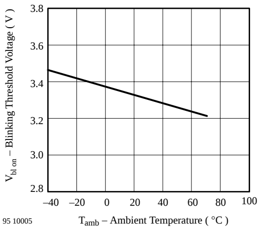
Figure 6. Blinking Threshold Voltage vs. Amb. Temperature
