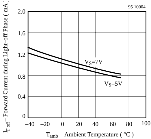
Figure 5. Forward Current (Light Off) vs. Amb. Temperature
