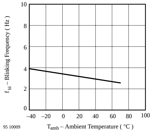
Figure 8. Blinking Frequency vs. Ambient Temperature
