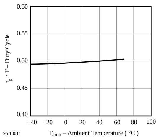
Figure 10. Duty Cycle vs. Ambient Temperature
