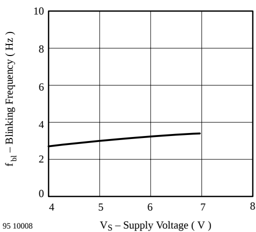
Figure 7. Blinking Frequency vs. Supply Voltage
