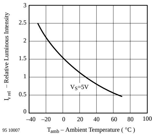
Figure 12. Relative Luminous Intensity vs. Amb. Temperature
