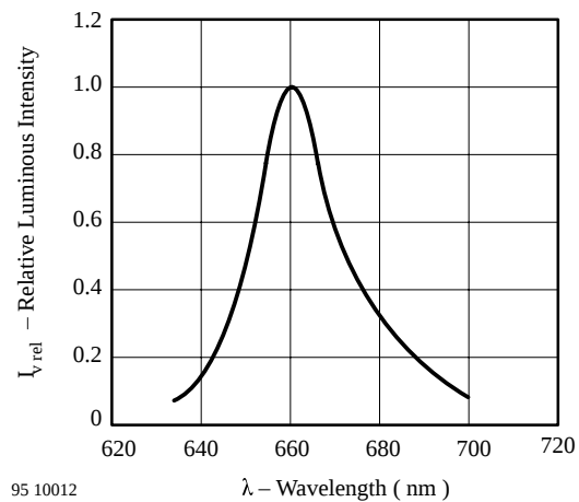
Figure 13. Relative Luminous Intensity vs. Wavelength
