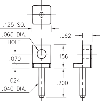
3621-0-32-XX-00-00-08-0 Board edge rivet mount
