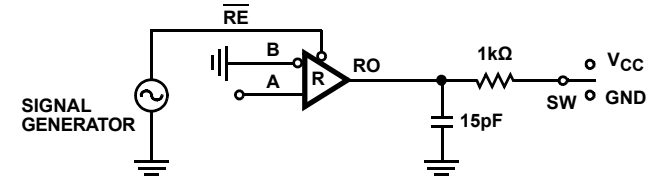
FIGURE 9. RECEIVER PROPAGATION DELAY AND DATA RATE
