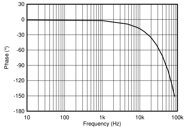
Figure 8-10. Normalized Phase, All Variants
