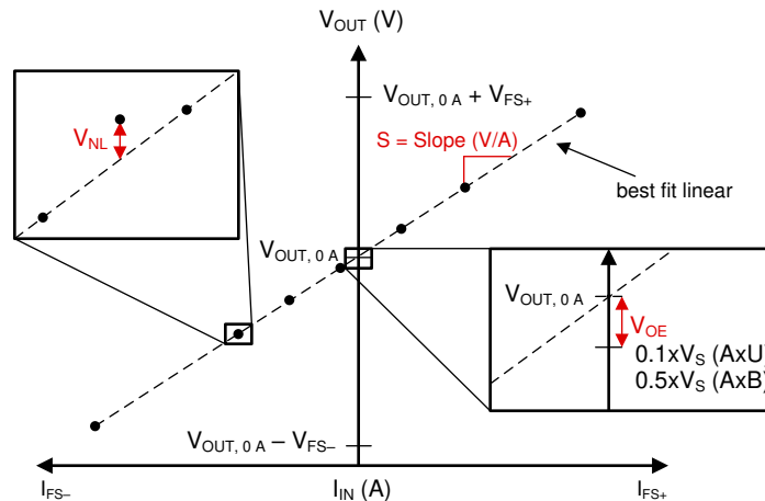
Figure 7-1. Sensitivity, Offset, and Nonlinearity Error
