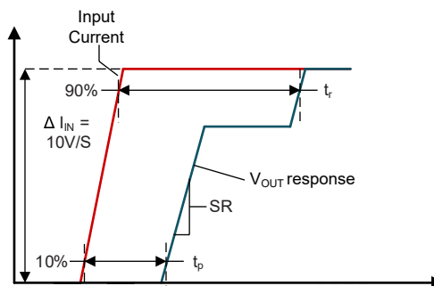
Figure 7-4. Current Overload Transient Response
