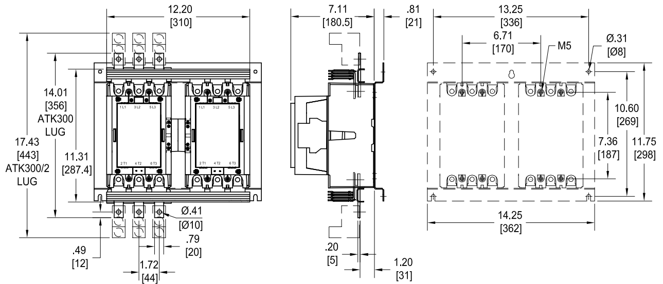
A/AF210, A/AF145 with mechanical interlock
