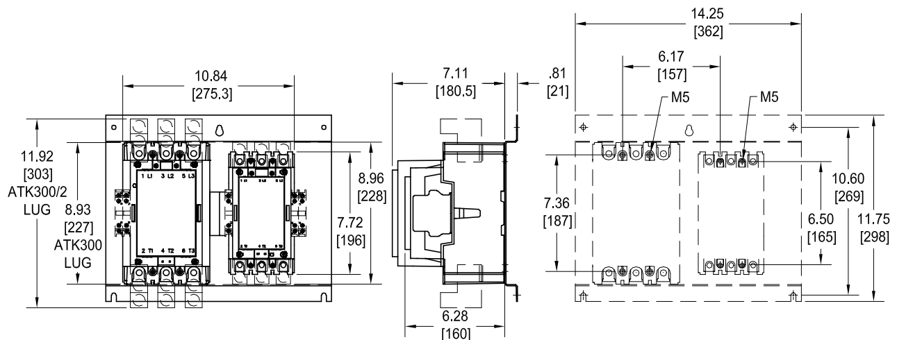
A/AF210, A/AF145 with mechanical interlock
