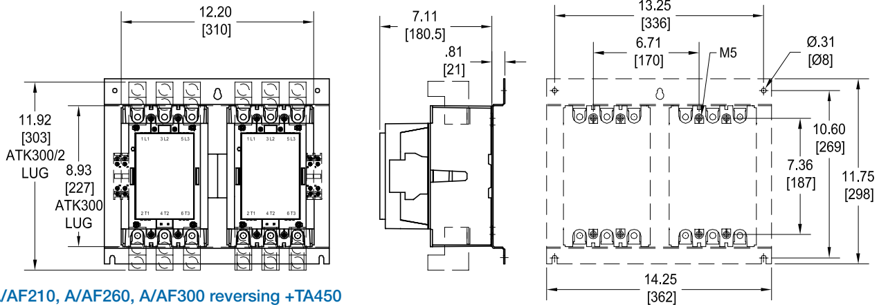
A/AF210, A/AF260, A/AF300 with mechanical interlock
