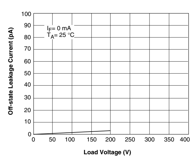
Figure 8. Leakage Current vs. Applied Voltage
