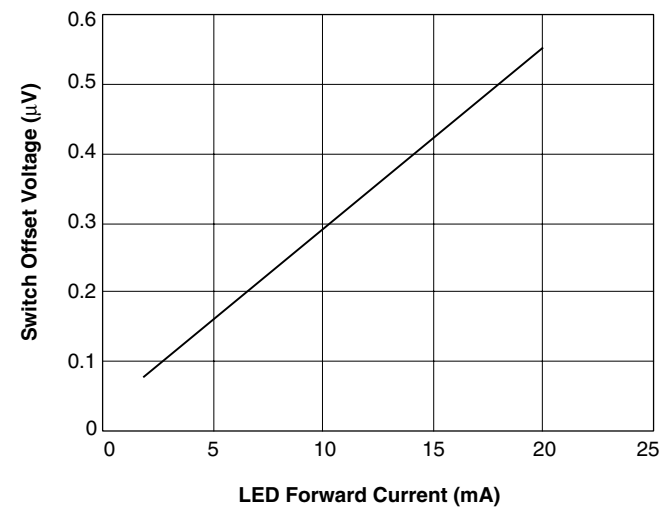
Figure 13. Switch Offset Voltage vs. LED Current
