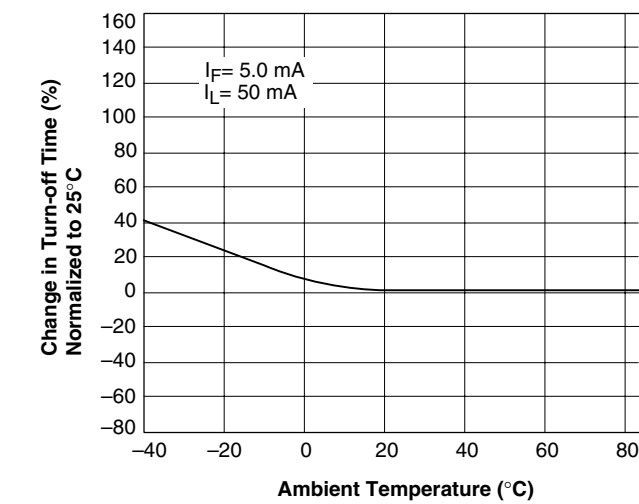
Figure 15. Turn-off Time vs. Temperature
