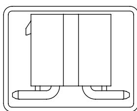
IPBT-1XX-H2-XX-D-XX SHOWN TUBE: PT-1-24-02-112 PLUG: TP-28
