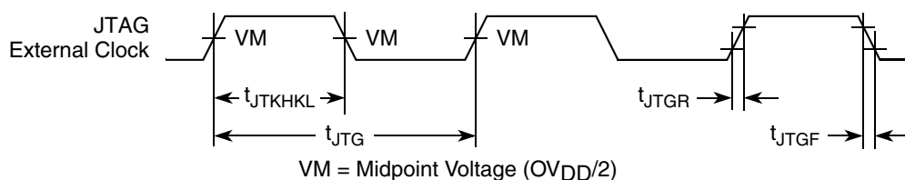
Figure 24. JTAG Clock Input Timing Diagram
