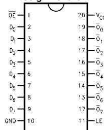
Pin Assignment for DIP
