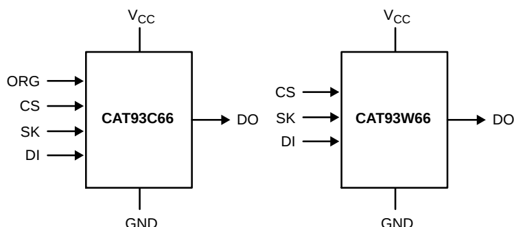
Figure 1. Functional Symbols
