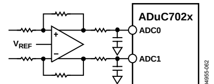
Figure 48. Buffering Differential Inputs
