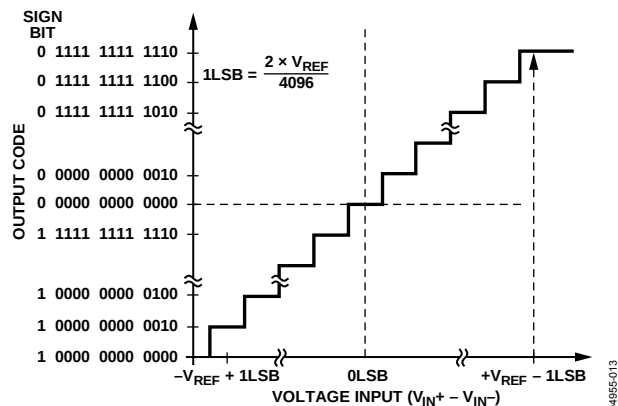
Figure 38. ADC Transfer Function in Differential Mode
