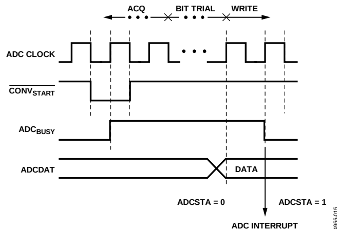
Figure 40. ADC Timing
