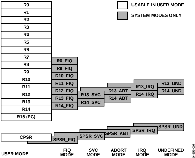
Figure 32. Register Organization
