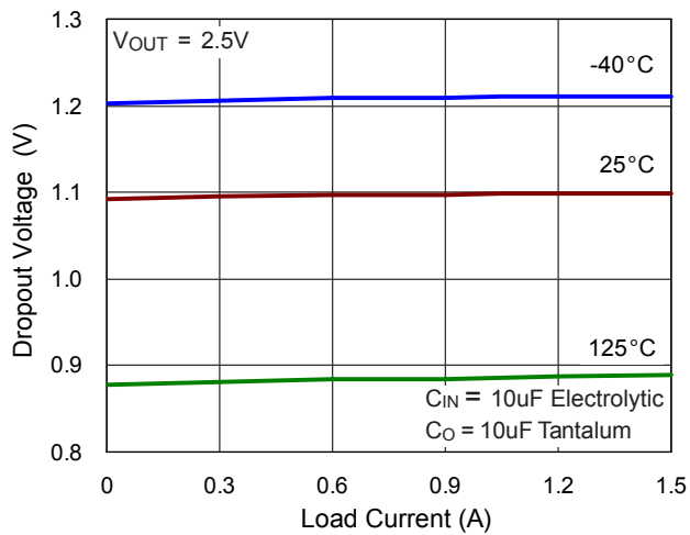
Dropout Voltage vs. I_O
