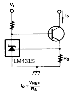
Figure 19. Constant-Current Sink
