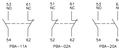
PBA-11A, PBA-02A & PBA-20A Front Mount Auxiliary Contact Blocks
