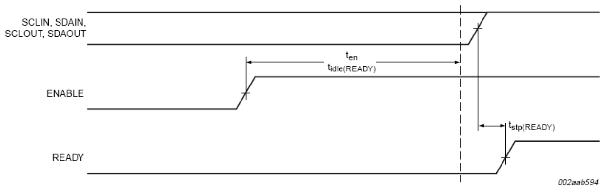
Figure 16. t_{stp}(READY) That Can Occur After t_{en}
