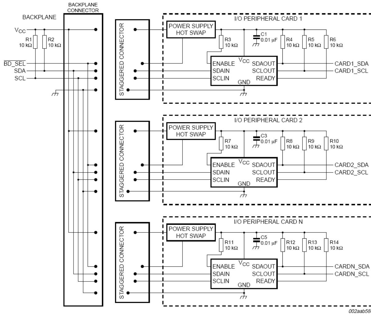
Figure 6. Hot Swapping multiple I/O Cards into a Backplane using the PCA9511A in a cPCI, VME and AdvancedTCA System
