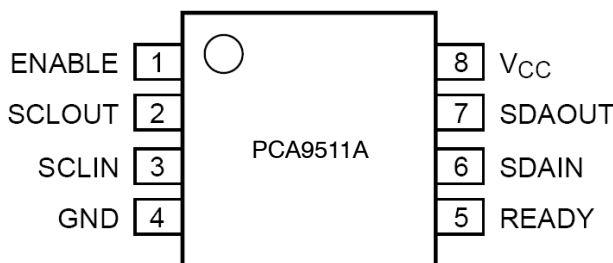
Figure 2. SOIC8 / Micro-8
