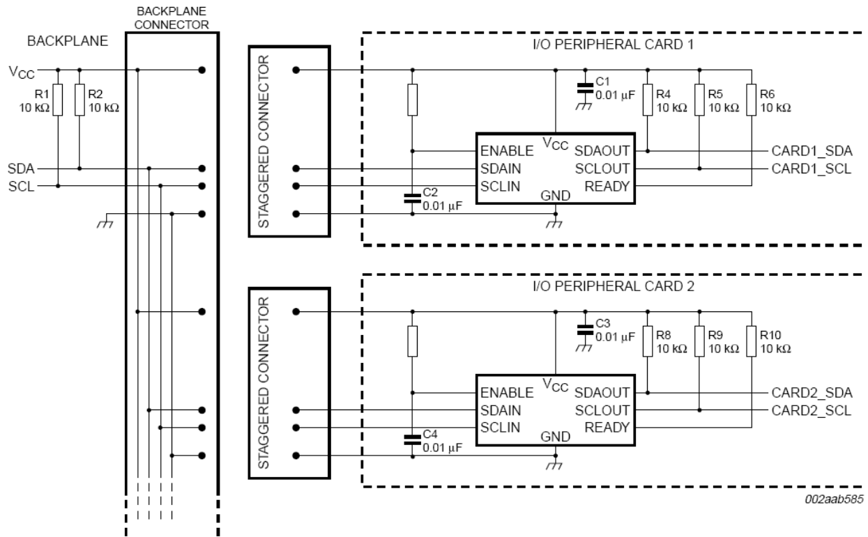
Figure 7. Hot Swapping Multiple I/O Cards into a Backplane Using the PCA9511A in a PCI System
