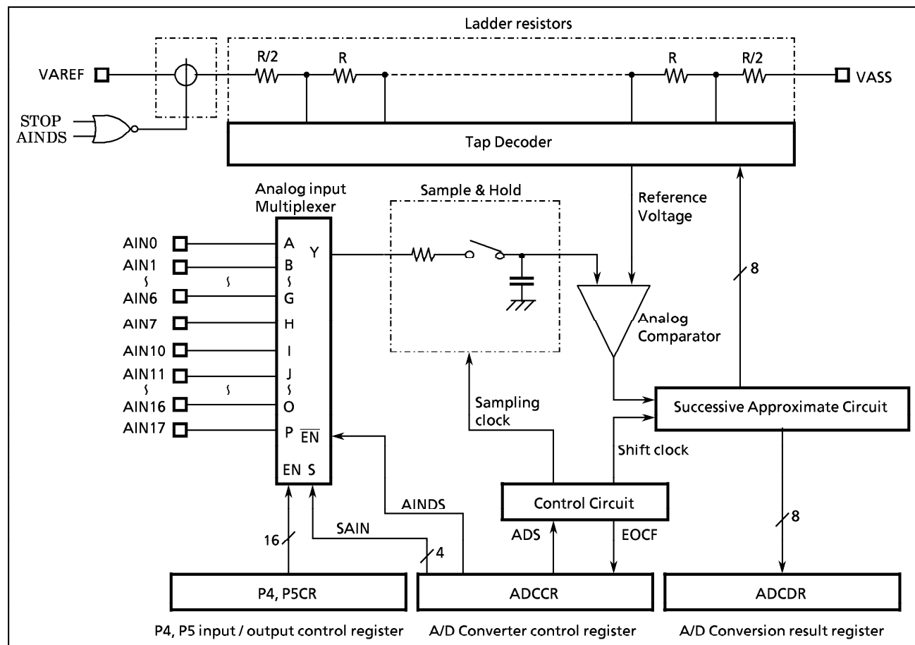
Figure 2-74. A/D Converter
