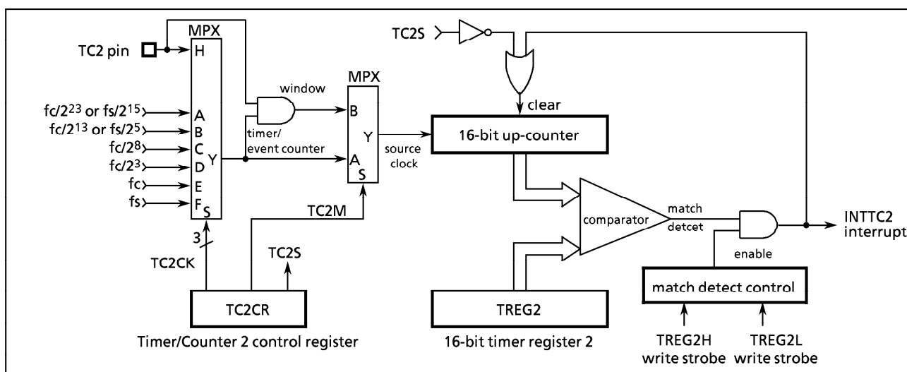
Figure 2-27. Timer/Counter 2 (TC2)
