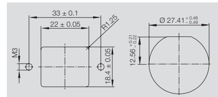
Standardised flange
