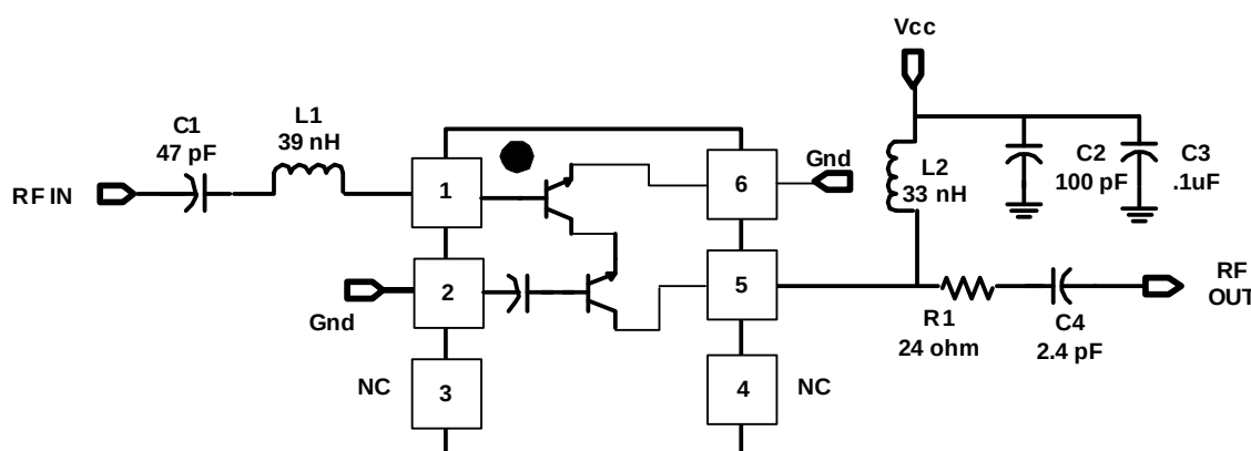
Figure 17. 434 MHz Application Schematic
