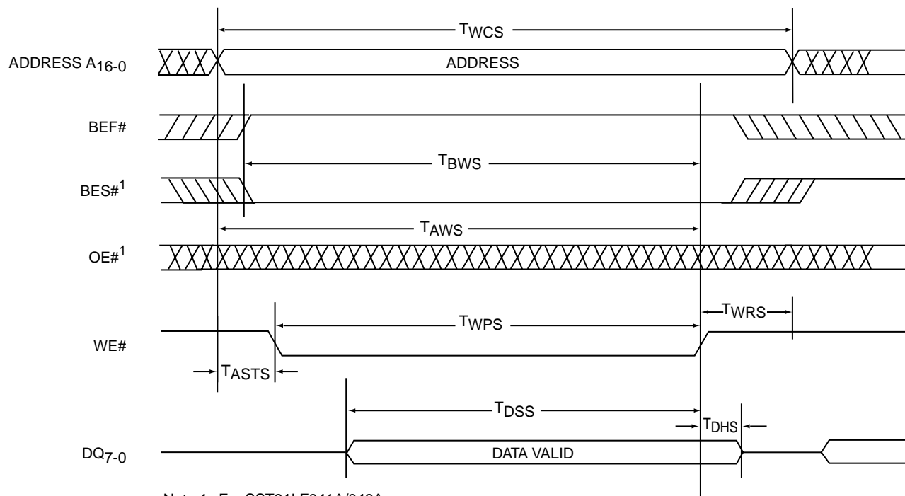
FIGURE 4: SRAM WRITE CYCLE TIMING DIAGRAM
