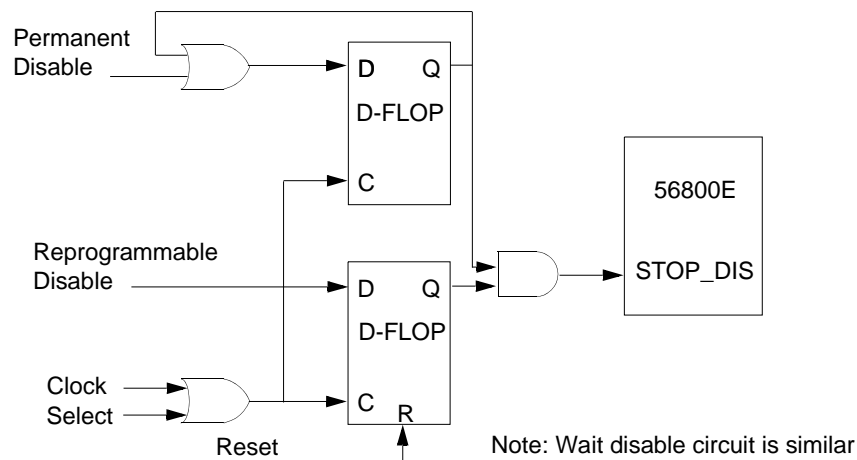
Figure 6-16 Internal Stop Disable Circuit
